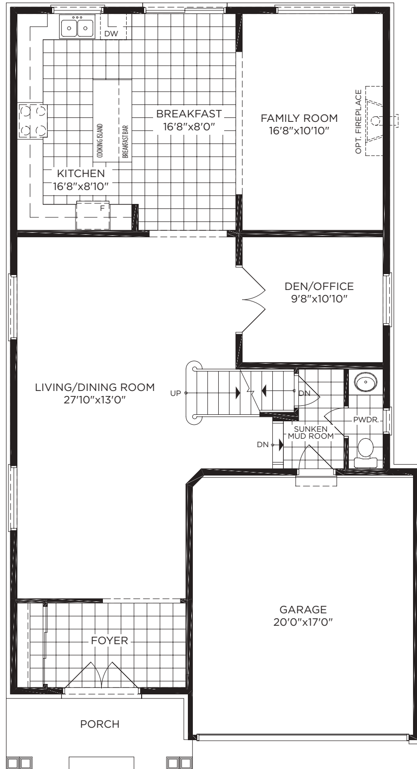
MAIN LEVEL
